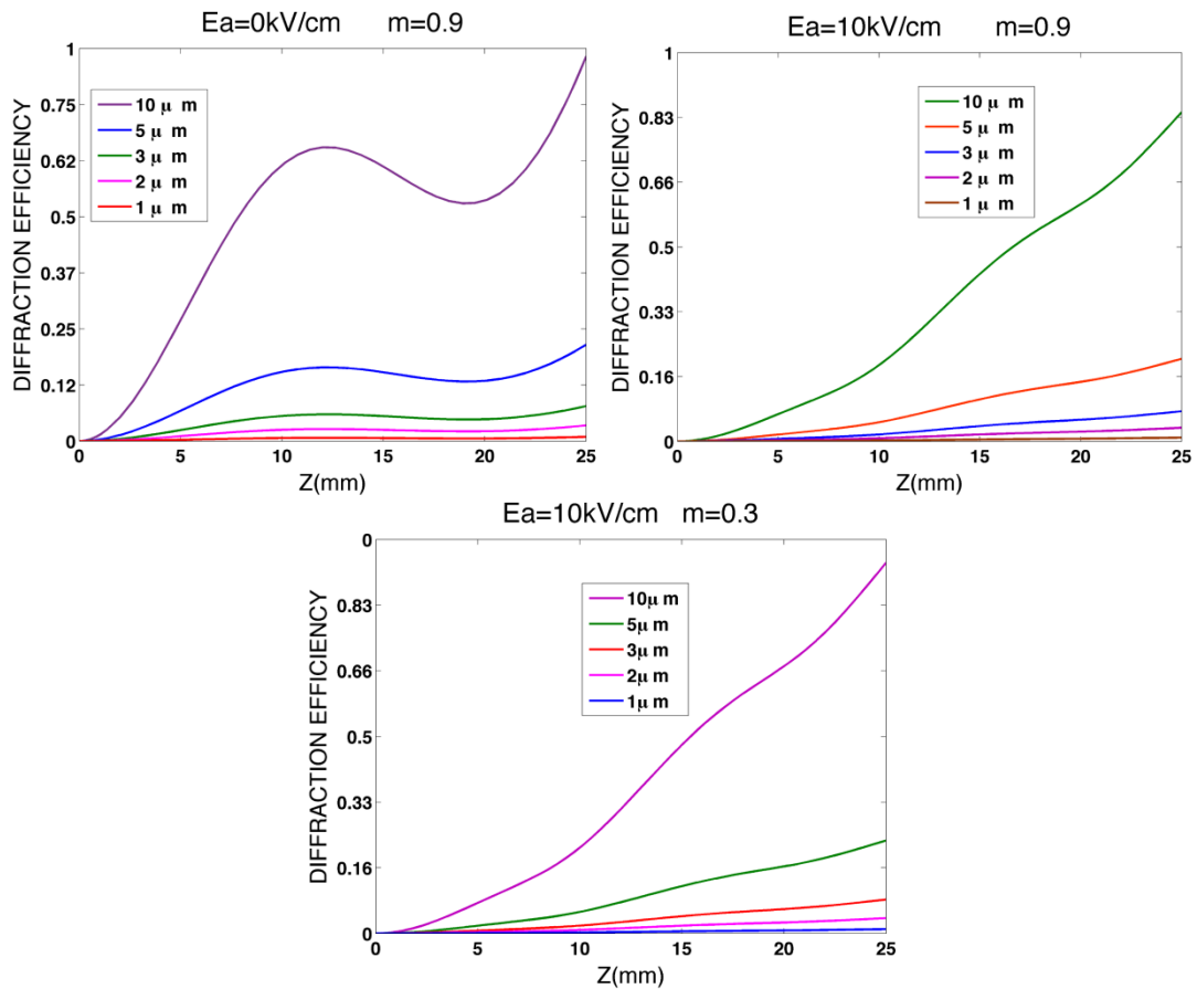
Fig. 3. BTO crystal diffraction efficiency in terms of the crystal thicknesses using red read-out light and different grating period: \Lambda=1\ \mu\text{m} , 2\ \mu\text{m} , 3\ \mu\text{m} , 5\ \mu\text{m} , 10\ \mu\text{m} , at various values of (a) m=0.9 , E_a=0\text{kV/cm} (b) m=0.9 , E_a=10\ \text{kV/cm} (c) m=0.3 , E_a=10\text{kV/cm}
