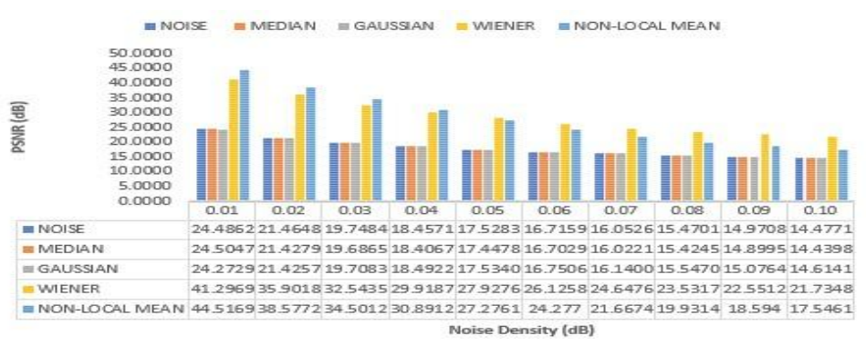
Fig. 10. Filters Comparison of SNR (dB) Values for Salt and Pepper Noise
