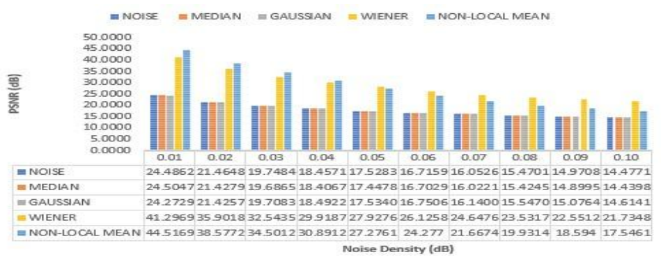
Fig. 9. Filters Comparison of PSNR (dB) Values for Salt and Pepper Noise
